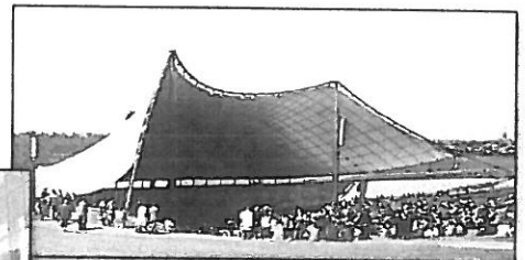
Membrane-Covered Cable Structure
